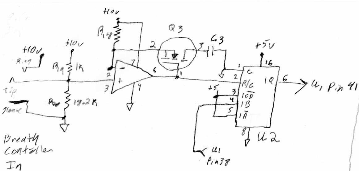
Breath Controller Circuit
